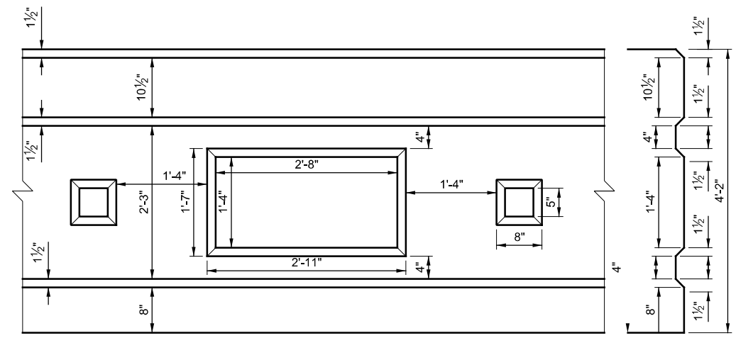
ELEVATION SECTION C-C PARAPET DETAIL
